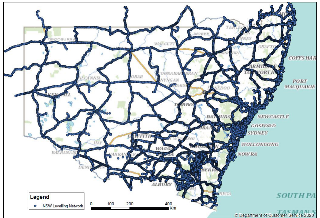
Figure 2: Location of benchmarks included in the NSW levelling adjustment. Courtesy DCS Spatial Services.
