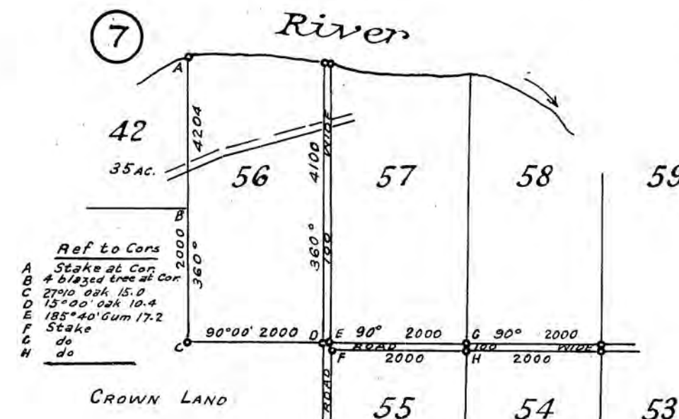
Part of original plan of Pors. 53 to 59 inclusive Survey dated 1860
