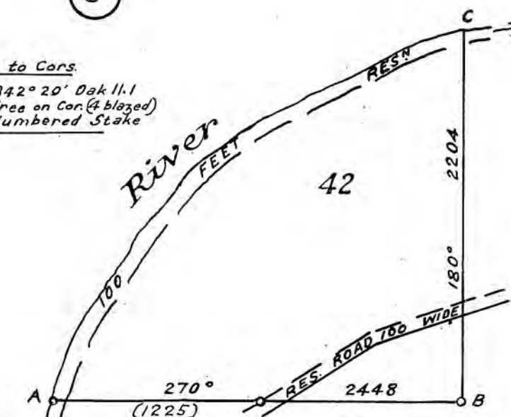
Original plan of Por. 42 - Survey dated 1859
