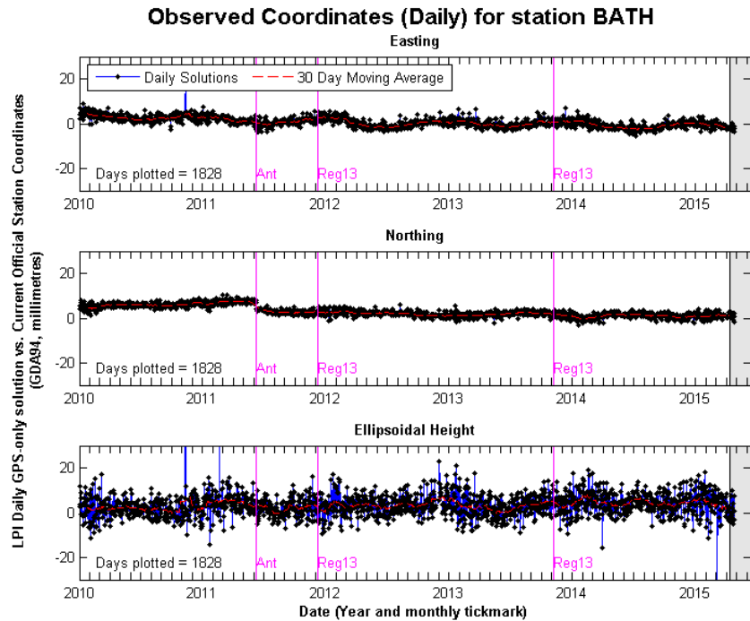
Figure 5: Observed position vs. official position of Bathurst CORS (LPI, 2015).
