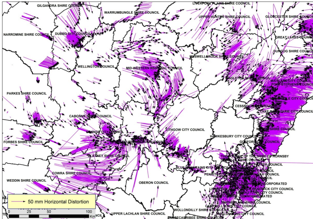
Figure 6: GDA94(1997) to GDA94(2010) horizontal distortion vectors at marks observed by GNSS, across the Central West, Sydney and Hunter regions of NSW.
