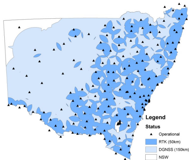
Figure 2: CORSnet-NSW backup redundancy map as of June 2015.
