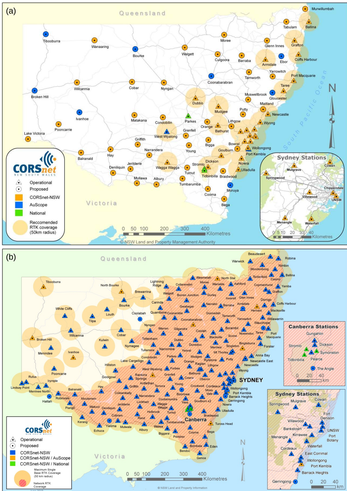
Figure 1: CORSnet-NSW network map as of (a) November 2009 and (b) June 2015.
