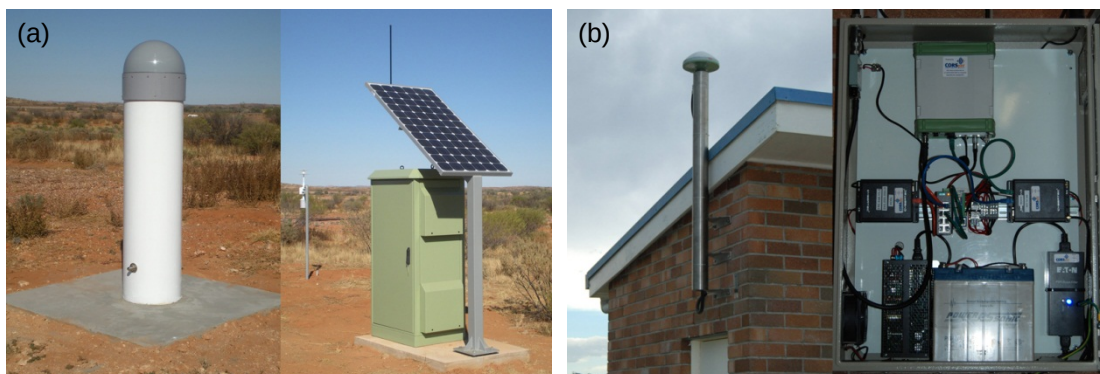
Figure 3: Typical CORSnet-NSW monumentation and auxiliaries at (a) Tier 2 and (b) Tier 3 sites.
